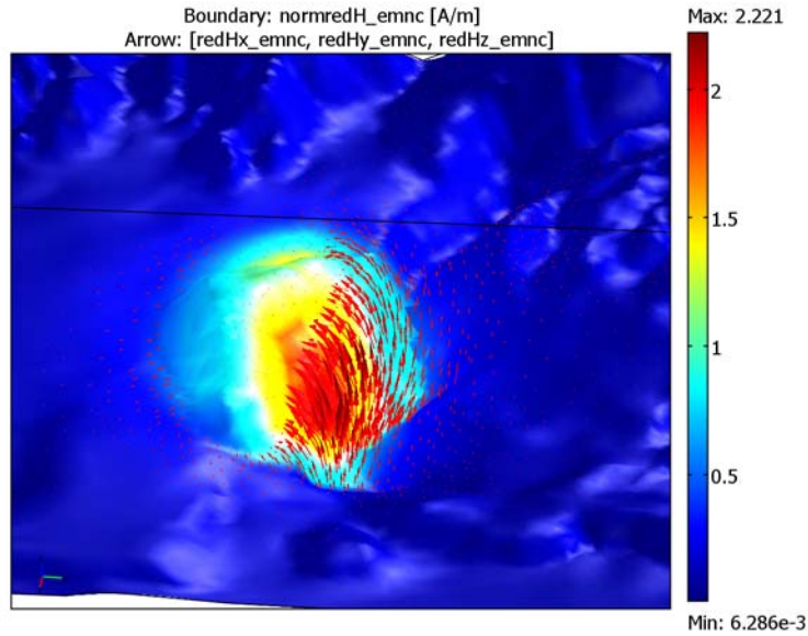
Figure 5-20: Boundary plot shows magnitude of reduced magnetic field on the surface of the Earth. Arrows show the direction and magnitude of reduced magnetic field on the surface of the Earth.
