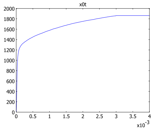
The time evolution of the armature velocity.
