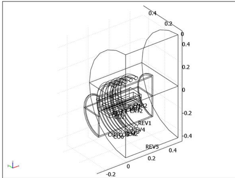
Figure 5-12: The furnace geometry cut in half. Note that you need model only one quarter of the full geometry due to symmetry.
