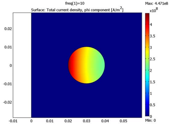
Figure 4-11: The current density at 10 Hz.
