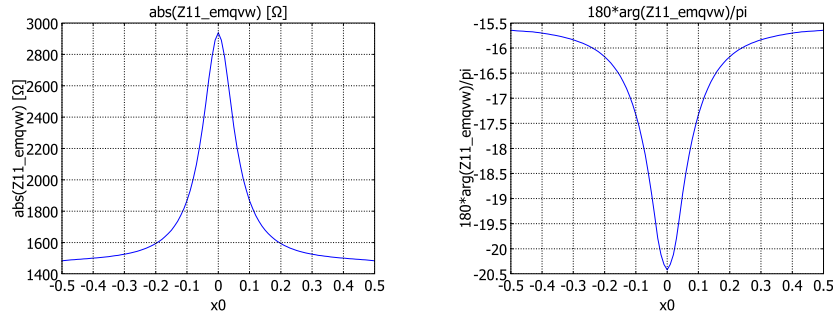
Figure 5-2: Absolute value and phase for the impedance as functions of air cavity coordinate. The peaks occur when the cavity is beneath the electrode.
