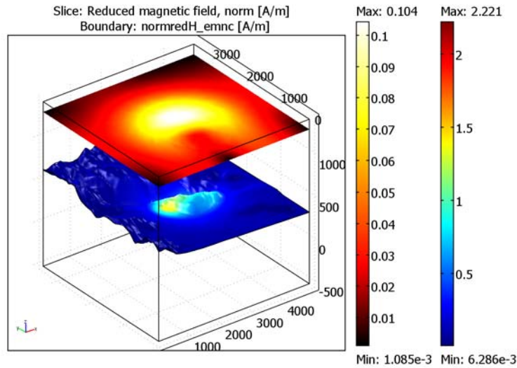
Figure 5-19: The slice color plot shows perturbations of magnetic intensity (norm of reduced magnetic field) at an altitude 1300 m. The boundary plot shows the same quantity on the ground.
