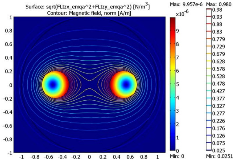
Figure 2-3: Force density and magnetic field.
