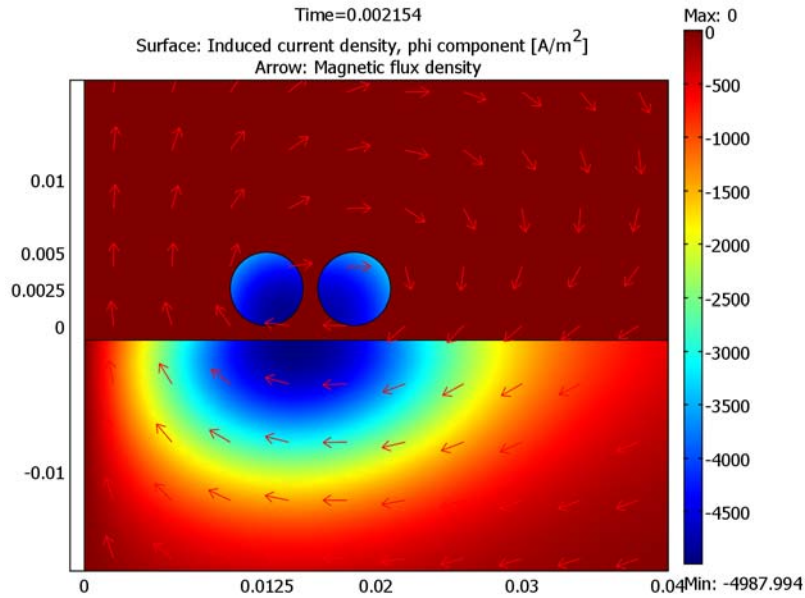
Figure 4-5: Induced current density and magnetic flux density for the transient solution.
