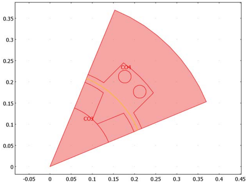
Figure 3-7: The smallest possible sector model.
