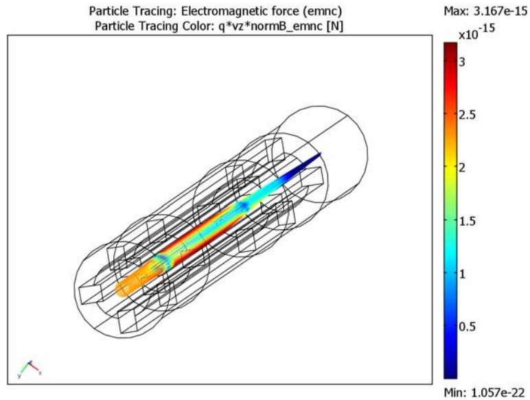
Figure 5-9: Particle tracing plot of the ions. The line colors show the local force acting on each ion. The force grows larger (red) far away from the center of the beam line and smaller (blue) where two oppositely polarized quadrupoles join.
