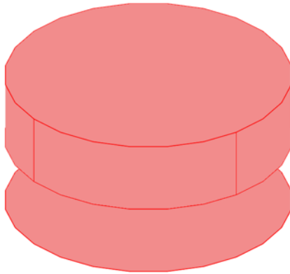
Figure 5-3: A cylindrical magnet above a \mu -metal plate is modeled.
