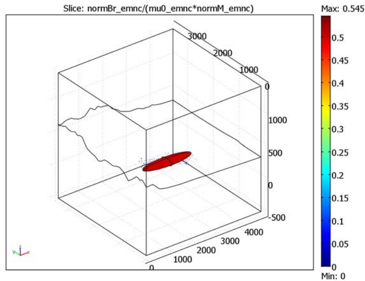
Figure 5-22: Slice plot of the dimensionless ratio of remanent to induced magnetizations inside the iron ore body at an elevation of 200 m above sea level. The two contributions to the magnetic anomaly are of comparable magnitude.
