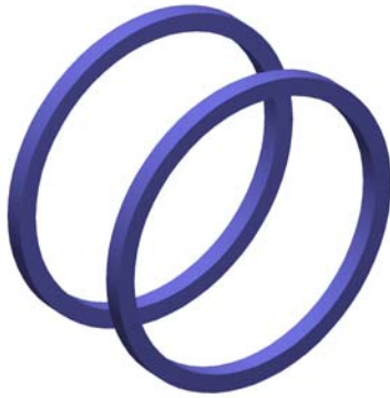
Figure 4-7: The Helmholtz coil consists of two coaxial circular coils, one radius apart along the axial direction. The coils carry parallel currents of equal magnitude.
