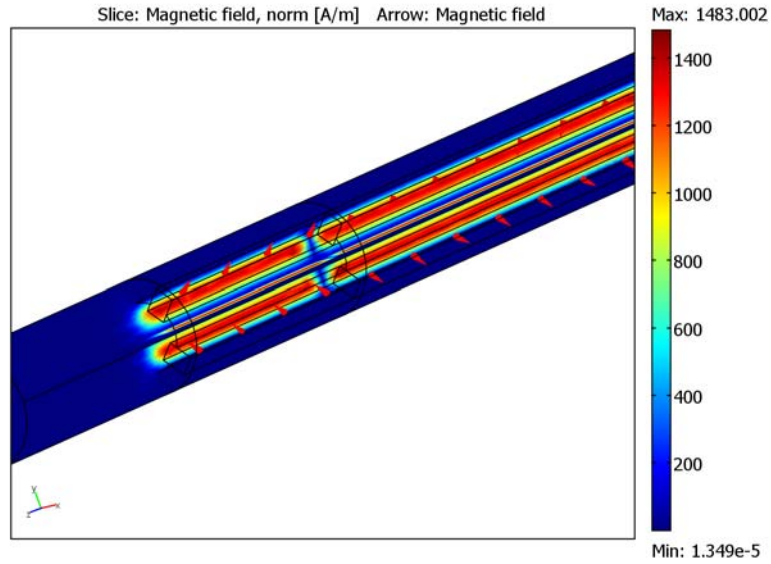
Figure 5-8: Slice plot and arrows of the magnetic field density in the quadrupole lens.
