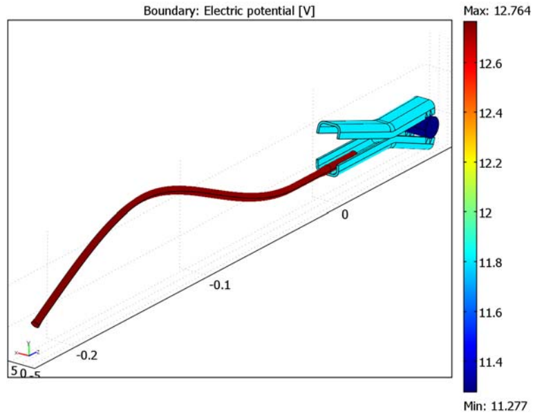
Figure 4-23: The potential distribution of the cable on the plus side of the battery. Almost the entire voltage drop is over the two junctions.
