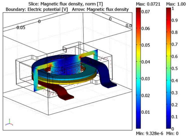
Figure 4-17: The final plot of the power inductor, showing the potential on the coil, the magnitude of the flux density inside the ferrite core, and the direction of the same as arrows.
