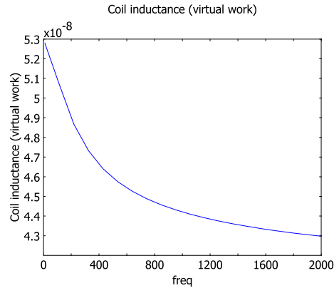
Figure 4-13: The inductance as a function of the frequency calculated using the virtual work method.
