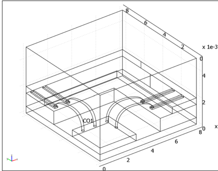
Figure 4-19: The model geometry, which studies the corner of an IC where four bonding wires connect a chip to a package.
