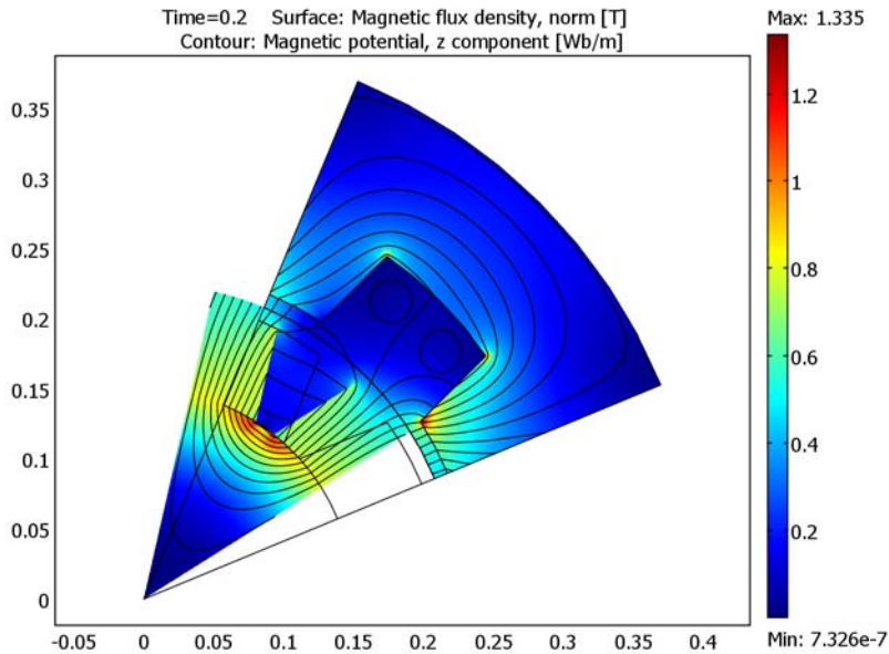
Figure 3-9: Magnetic flux norm (surface) and field lines (contours) at t=0.2 s.
