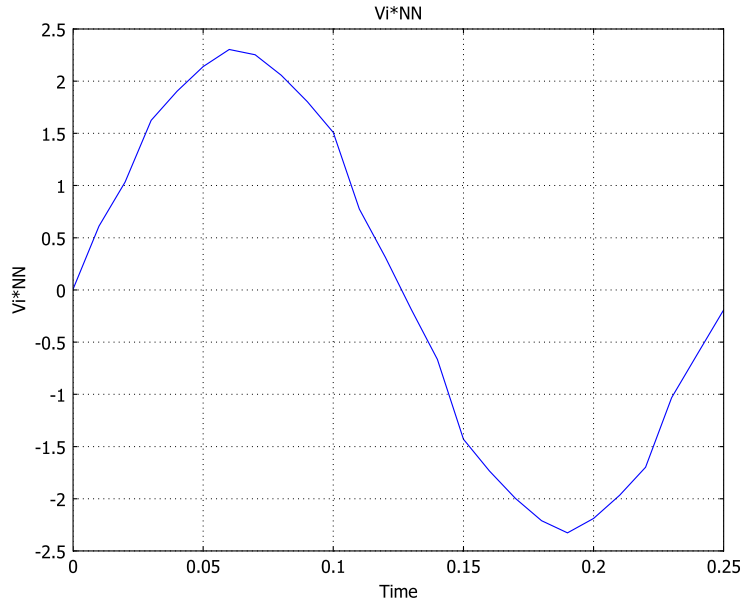
Figure 3-4: The generated voltage over one quarter of a revolution. This simulation used a single-turn winding.
