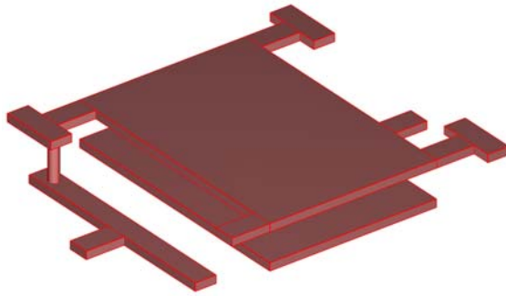
Figure 4-1: The tunable MEMS capacitor consists of two metal plates. The distance between the plates is tuned via a spring connected to one of the plates.
