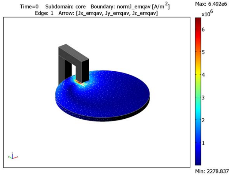
The eddy current magnitude and direction at t = 0 s.
