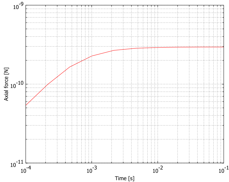
Figure 4-6: Resultant repulsive axial Lorentz force (N) between the coils and the plate vs. time (s).
