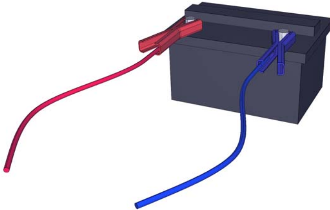
Figure 4-21: A view of the entire system, where the cables, clips, and poles are modeled in a physical model. All other components are modeled as circuit models.
