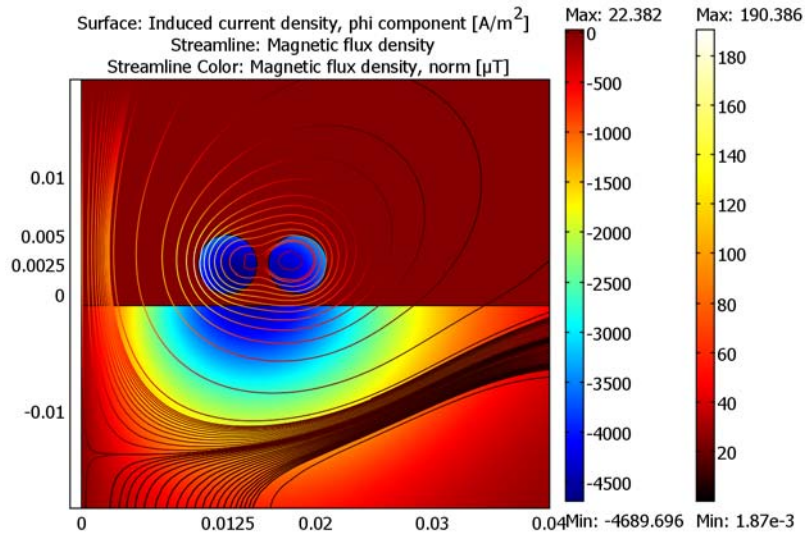
Figure 4-4: The \phi component of the induced current density for the time-harmonic solution plotted together with the field lines of the magnetic flux.
