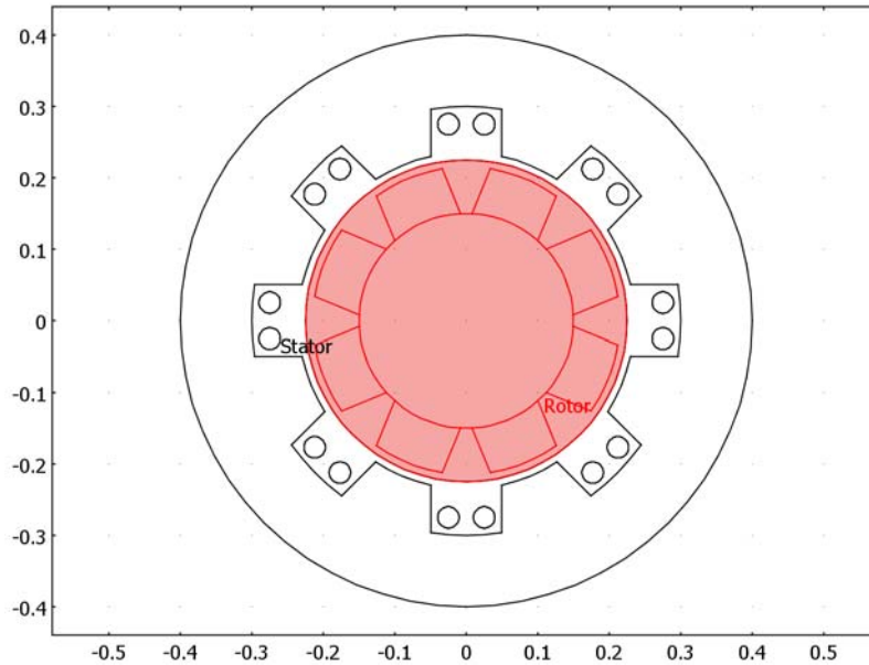
Figure 3-6: Generator geometry.
