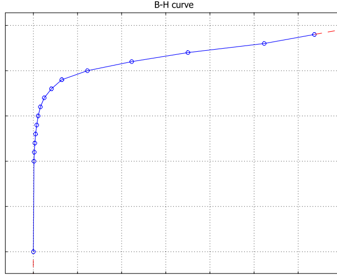
Figure 3-3: The norm of the magnetic flux, |\mathbf{B}| , versus the norm of the magnetic field, |\mathbf{H}| , for the rotor and stator materials. The inverse of this curve is used in the calculation.
