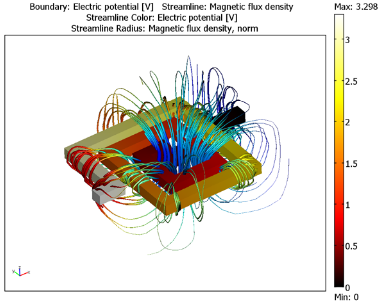
Figure 4-16: Electric potential in the device and magnetic flux lines around the device.
