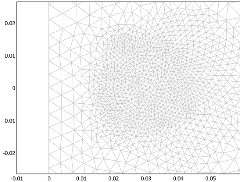
The mesh for the inductance computation.
