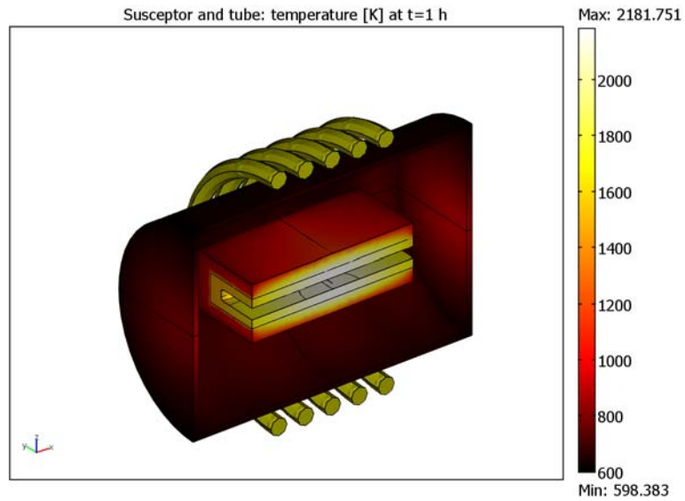
Figure 5-15: Temperature distribution for the important parts of the furnace after 1 hour of heating. The coils are plotted only to show their location; there is no temperature information on their surfaces.
