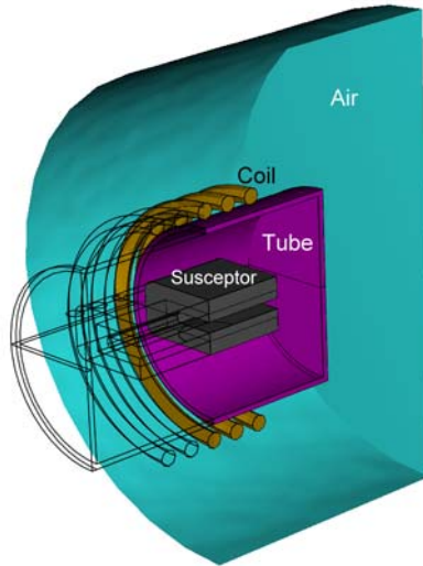
Figure 5-13: The part of the geometry included in the simulation, also with the surrounding air domain.
