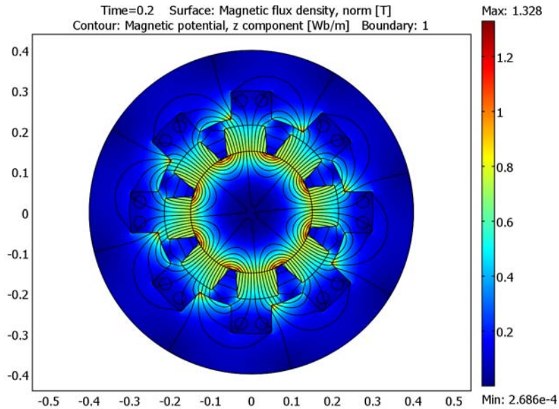
Figure 3-5: The norm and the field lines of the magnetic flux after 0.2 s of rotation. Note the brighter regions, which indicate the position of the permanent magnets in the rotor.
