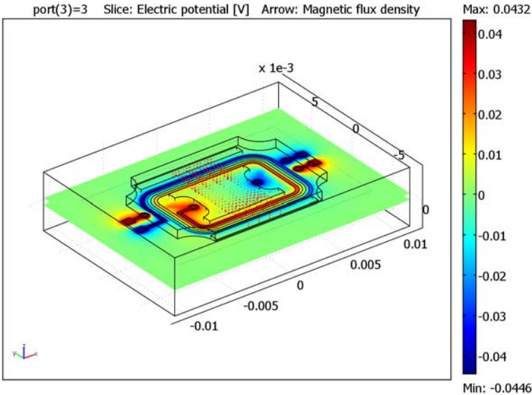
Figure 4-18: The plot shows the electric potential for the two coil layers and the magnetic flux density as arrows.
