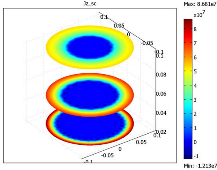
Figure 5-11: The current density at t = 0.02 , 0.05 , and 0.1 . The swelling of the ring comes from the transition out of the superconducting state at current densities exceeding J_C .
