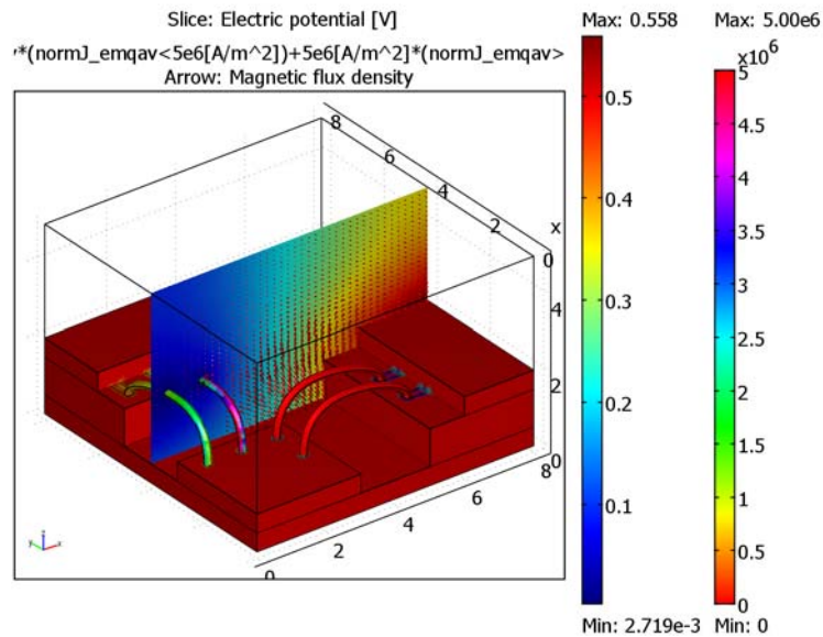
Figure 4-20: This plot shows a slice plot, an arrow plot of the magnetic flux density, and a boundary plot of the current density. For this solution, the third bonding wire is used as input, giving the third column in the parameter matrix.
