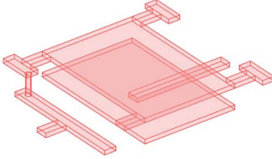
Figure 4-2: The computational domain. The interiors of the capacitor plates and the connecting bars are not included.
