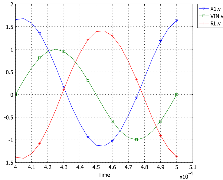
Figure 4-28: Input signal ( sim_VIN_v ), output signal ( sim_RL_v ), and inductor voltage ( sim_X1_v ) as functions of time.
