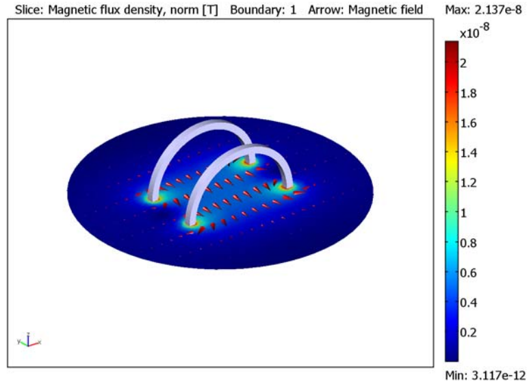
Figure 4-9: The surface color plot shows the magnetic flux density. The arrows indicate the magnetic field ( H ) strength and direction.
