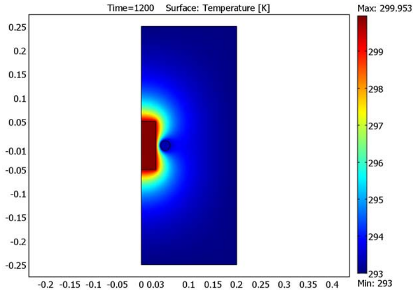
Figure 2-5: Temperature distribution in the cylinder and its surroundings after 1200 s.
