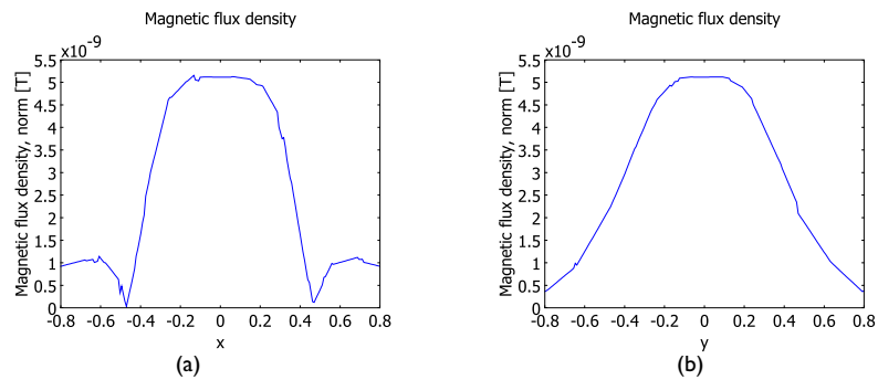
Figure 4-10: The magnetic flux density profile. The plots show the profile taken along a radial cross-sectional line through the axis right between the coils (a) and a profile taken along the axis (b). A high degree of uniformity is clearly shown.
