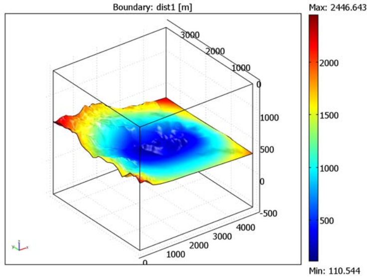
Figure 5-21: The boundary plot shows the approximate distance from the Earth's surface to the iron ore bed.
