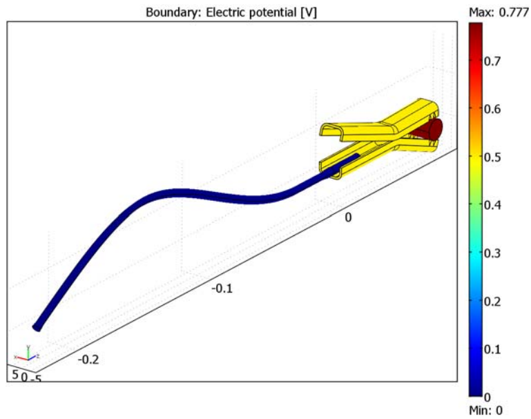
Figure 4-24: The potential distribution of the cable on the minus side of the battery.
