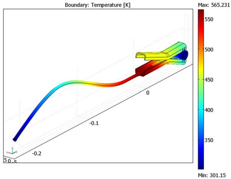
Figure 4-25: The temperature distribution on the plus side of the battery. The area around the cable-clip junction gets a high temperature that can damage a soldered junction.
