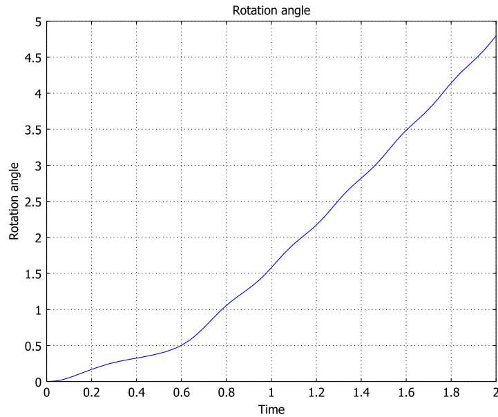
Figure 3-8: The time evolution of the rotation angle is shown. After about 1 s, the rotation angle increases linearly with time corresponding to constant rotation speed.
