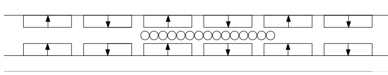
Figure 3-1: Cross section of the LEM's moving coil
