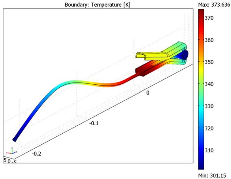
Figure 4-26: The temperature distribution on the minus side of the battery. The distribution is less critical here due to the alternative path for the current.
