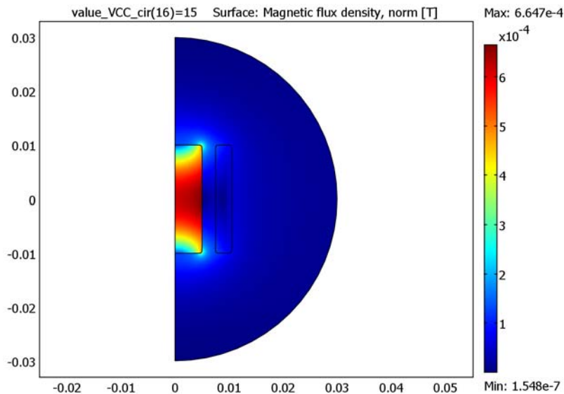
Figure 4-27: Magnetic flux density (color) after the bias point calculation.
