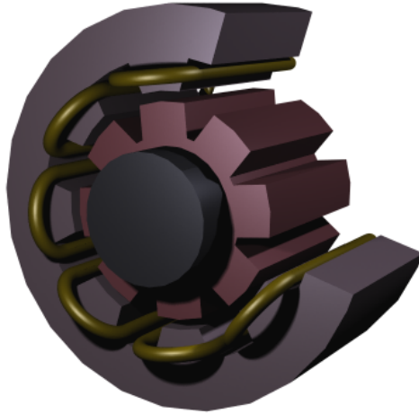
Figure 3-2: Drawing of a generator showing how the rotor, stator, and stator winding are constructed. The winding is also connected between the loops, interacting to give the highest possible voltage.
