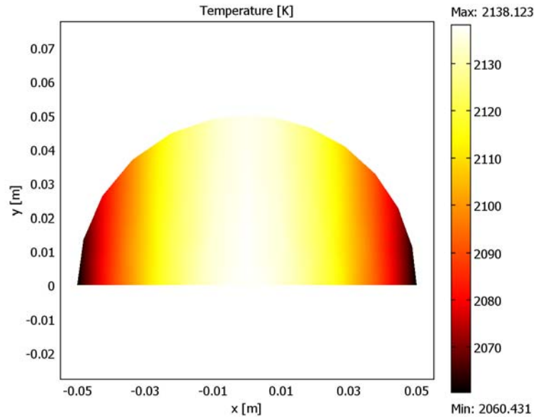
Figure 5-16: Temperature distribution across the surface of the wafer.
