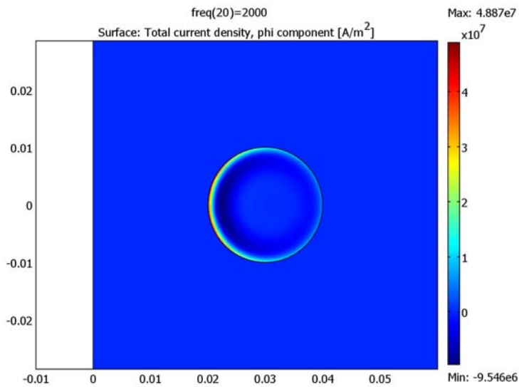
Figure 4-12: The current density at 2 kHz.
