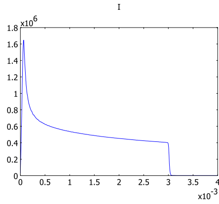
The time evolution of the rail current.
