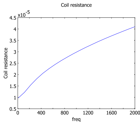
Resistance ( \Omega ) as a function of frequency (Hz).
