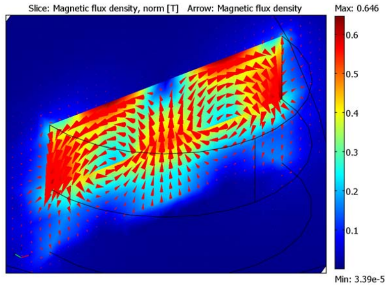
Figure 5-4: The magnetic flux density and direction is plotted in a cross section of the geometry. The one-sided behavior is clearly seen as the flux does not emerge on the top of the magnet.
