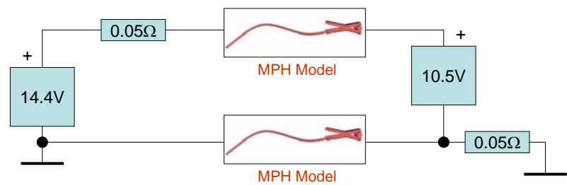
Figure 4-22: A block diagram over the entire charger system.
