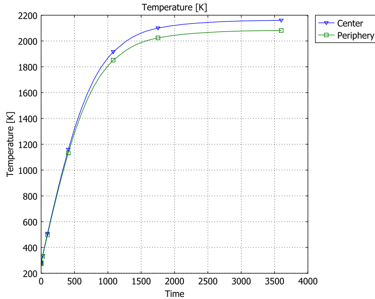
Figure 5-14: The temperature at two locations on the wafer during a heating cycle of one hour.
