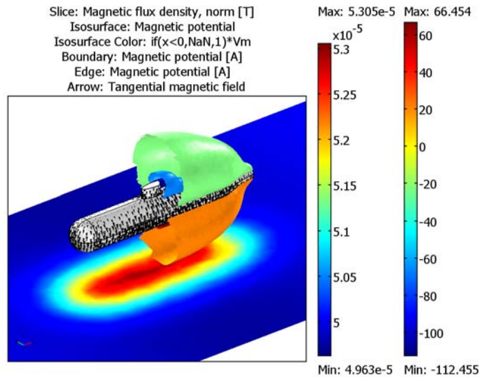
Figure 5-7: The slice color plot shows the total magnetic flux density (left color legend). The arrows show the direction and strength of the tangential magnetic field in the hull. The isolevels show the reduced magnetic potential (right color legend).
